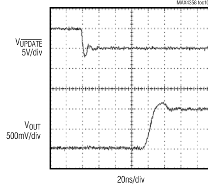
SWITCHING TIME
